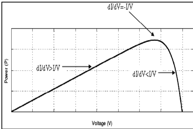
Fig. 7 : P-V curve of a PV cell
