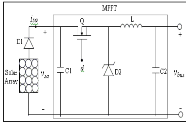
Fig. 2 : Circuit schematic of the photovoltaic power subsystem
