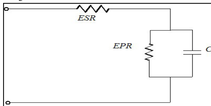
Fig.6 : Electrical equivalent of Ultra capacitor
