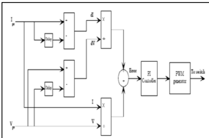
Fig.8 : Block diagram of IC algorithm in MATLAB/Simulink
