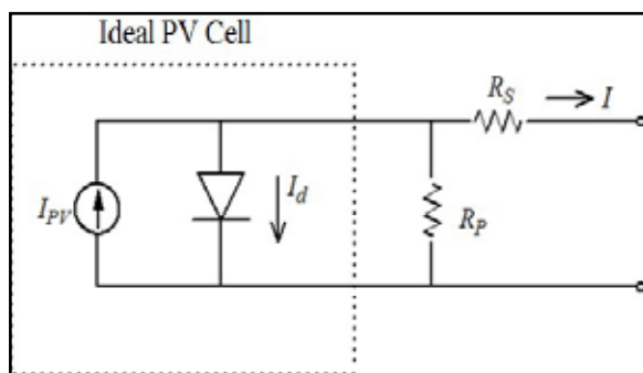
Fig.4 : Photovoltaic model
