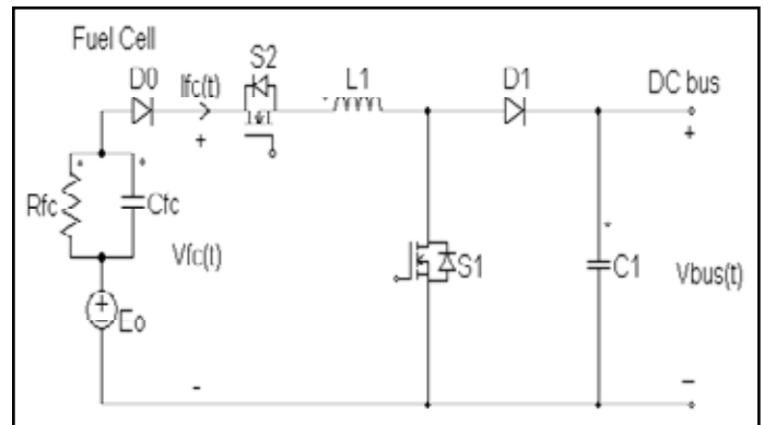
Fig. 3 : Circuit schematic of the fuel cell power subsystem.
