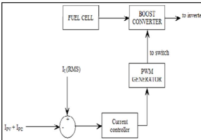
Fig. 9. Current control strategy for power balance
