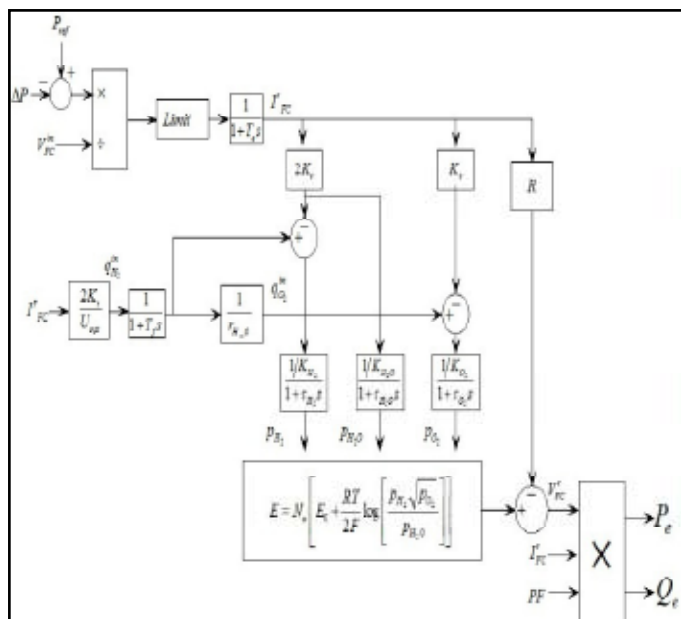
Fig.5 : Dynamic modeling of PEMFC
